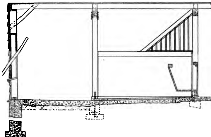
FIG. 180.—CROSS SECTION THROUGH HORSE BARN
